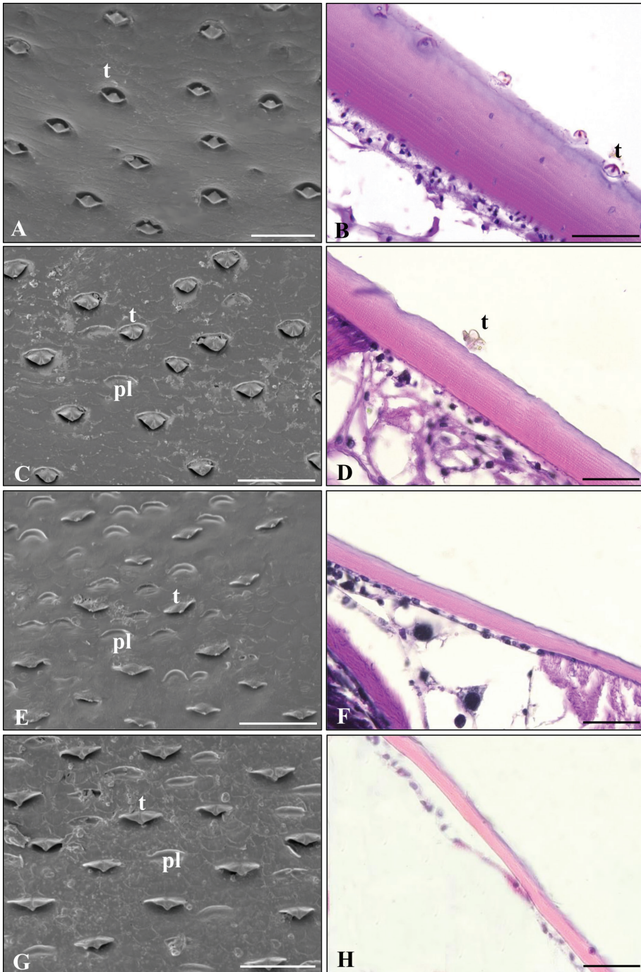
Figure 8. Scanning electron ( A, C, E, G ) and light microscope ( B, D, F, H ) micrographs on the studied Armadillidium species' tergites. Armadillidium vulgare ( A, B ), A. versicolor ( C, D ), A. nasatum ( E, F ), A. zenckeri ( G, H ). Abbreviations: pl – plaques, t – tricorn receptor. Staining: hematoxylin-eosin (HE) – B, D, F, H . Scale bars: 50 \mu m.
