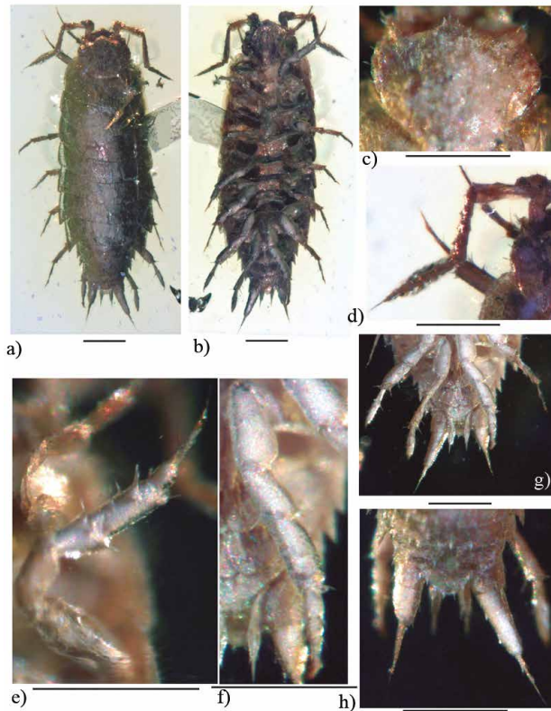
Figure 1. Palaolibrinus spinicornis gen. nov. sp. nov., ♂ adult holotype (IHNFG-4984); (a, b) General habitus, dorsaland ventral views; (c) Cephalon in dorsal view; (d) Antenna; (e) Pereiopod II; (f) Pereiopod VII; (g) Pleopod 2-5; (h) Pleotelson with uropods, dorsal view. holotype in dorsal view. Scale bars = 200 \mu m.
