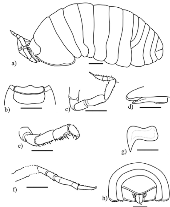
Figure 6. Palaeospherarmadillo mazanticus gen. nov. sp. nov., ♂ adult holotype (IHNF-4997); (a) General habitus, lateral view; (b) Cephalon in dorsal view; (c) Antenna; (d) Lateral margin of first coxal plate in ventral view; (e) Pereiopod I; (f) Pereiopod VII; (g) Pleopod 3; (h) Pleotelson with uropods, dorsal view. Scale bars = 200 µm.
