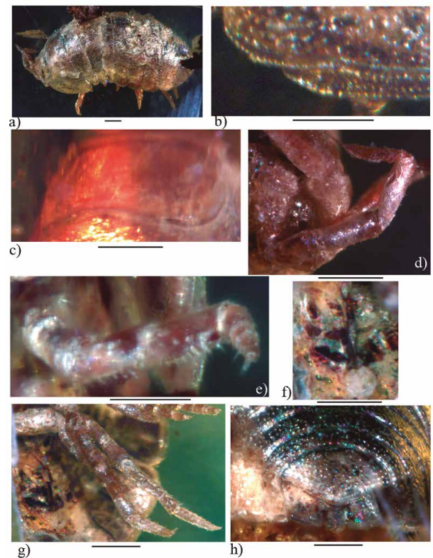
Figure 5. Palaeospherarmadillo mazanticus gen. nov. sp. nov., ♂ adult holotype (IHNF-4997); (a) General habitus, lateral view; (b) Lateral margin of first coxal plate in ventral view; (c) Cephalon in dorsal view; (d) Antenna; (e) Pereiopod I; (f) Pleopod 3; (g) Pereiopod VII; (h) Pleotelson with uropods, dorsal view. Scale bars = 200 µm.
